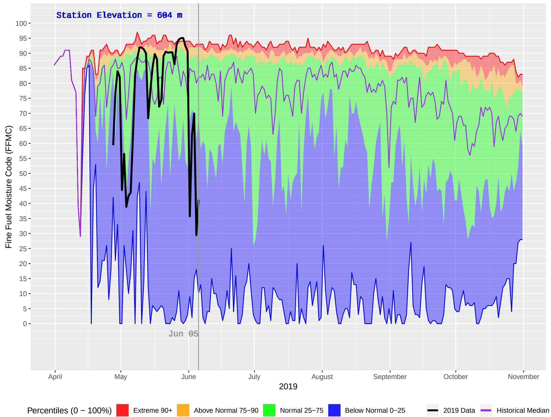
NELSON FORKS (119) : Historical (1986–2018) and Current (2019) Daily Fine Fuel Moisture Code (FFMC)
