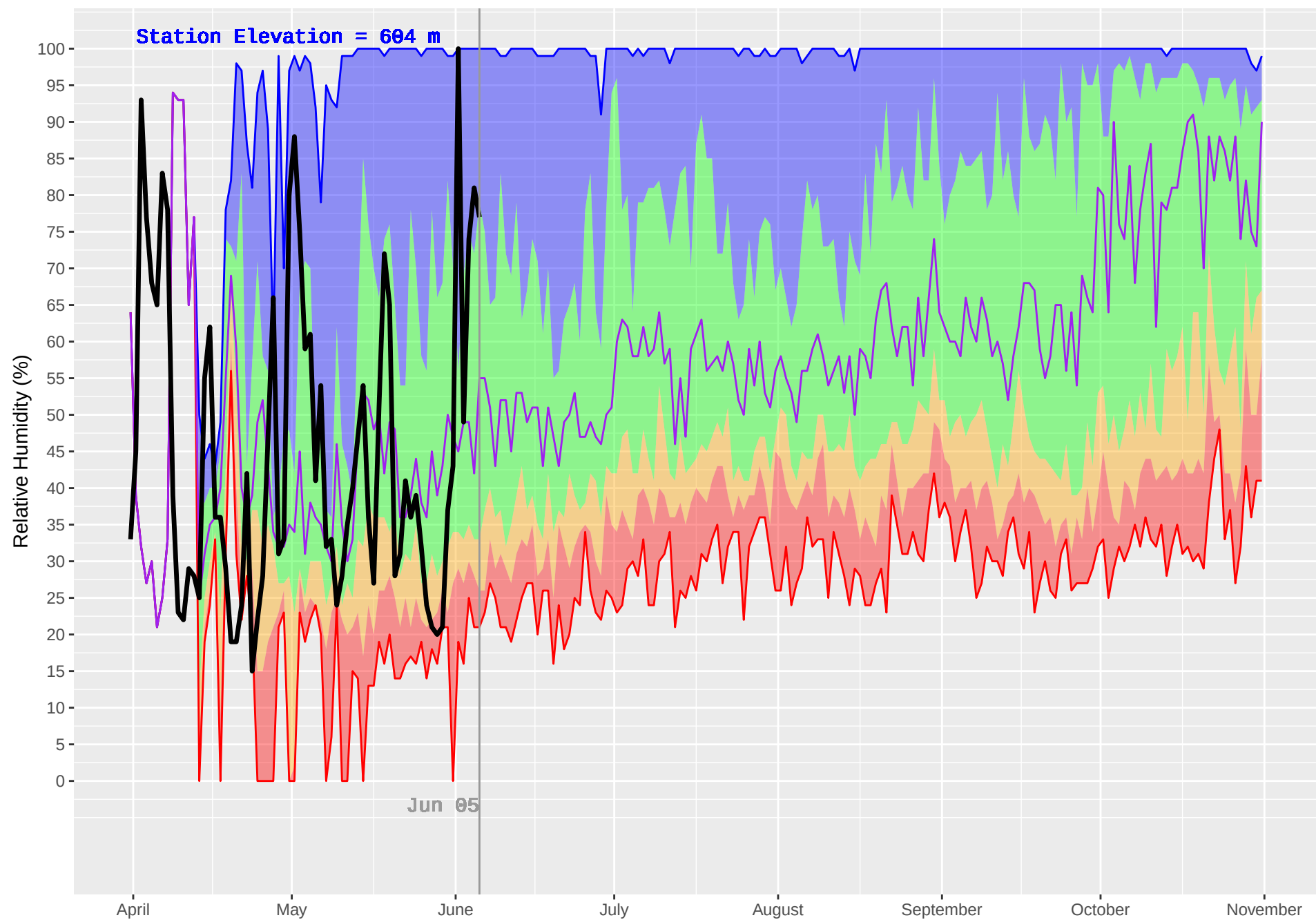
NELSON FORKS (119) : Historical (1986–2018) and Current (2019) Daily Relative Humidity
