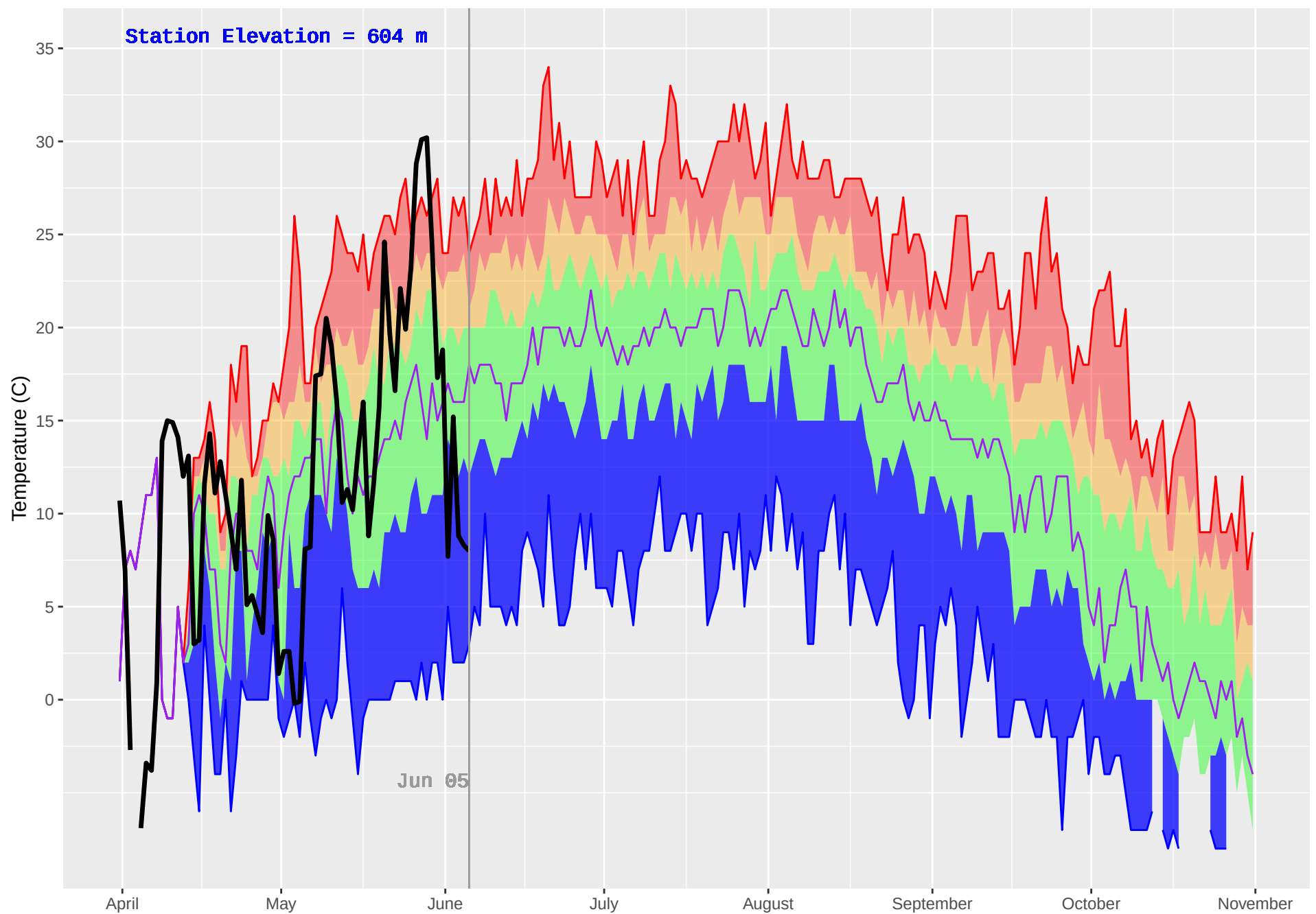
NELSON FORKS (119) : Historical (1986–2018) and Current (2019) Daily Temperature
