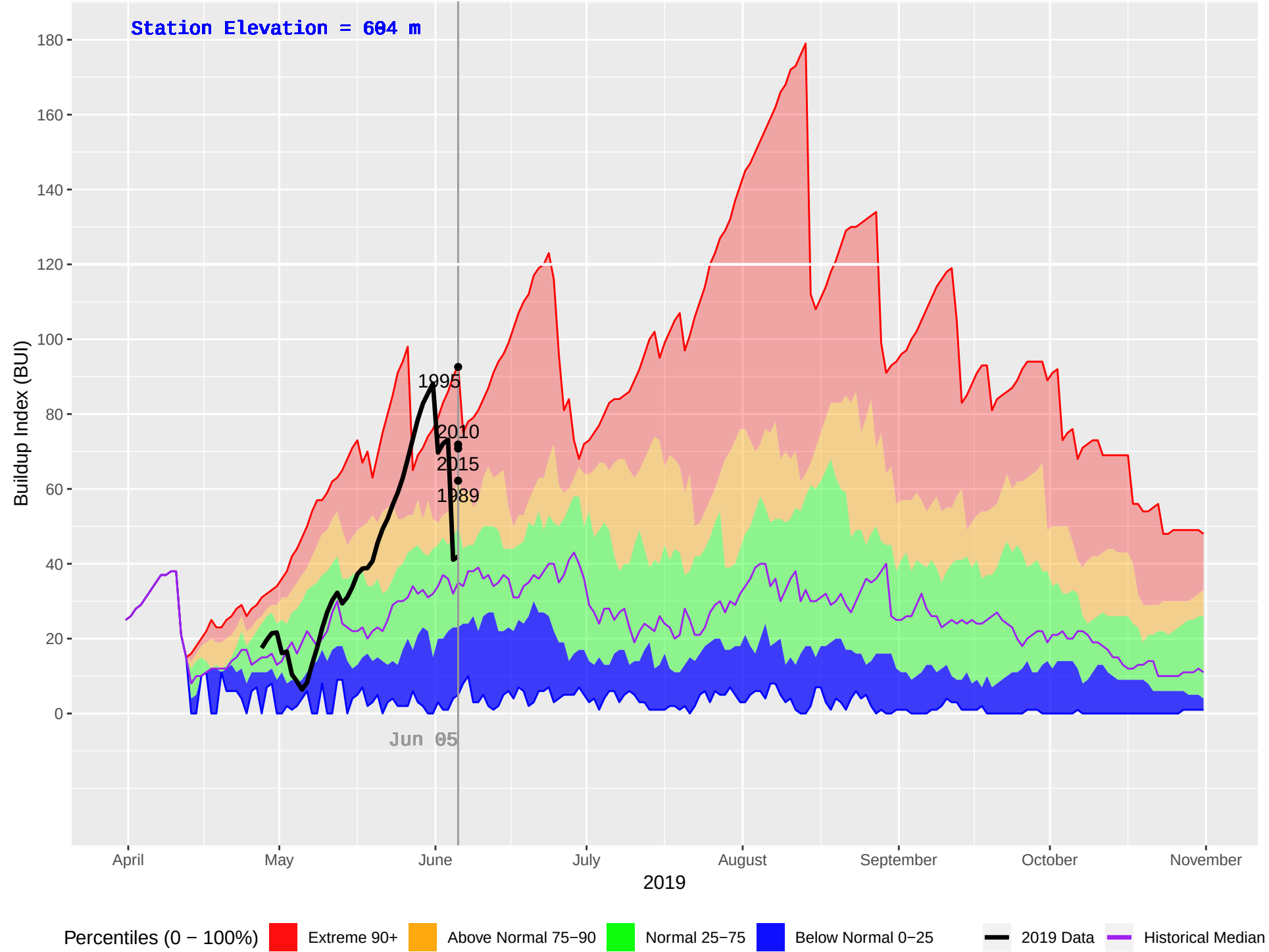
NELSON FORKS (119) : Historical (1986–2018), Current (2019) Daily Buildup Index (BUI)
