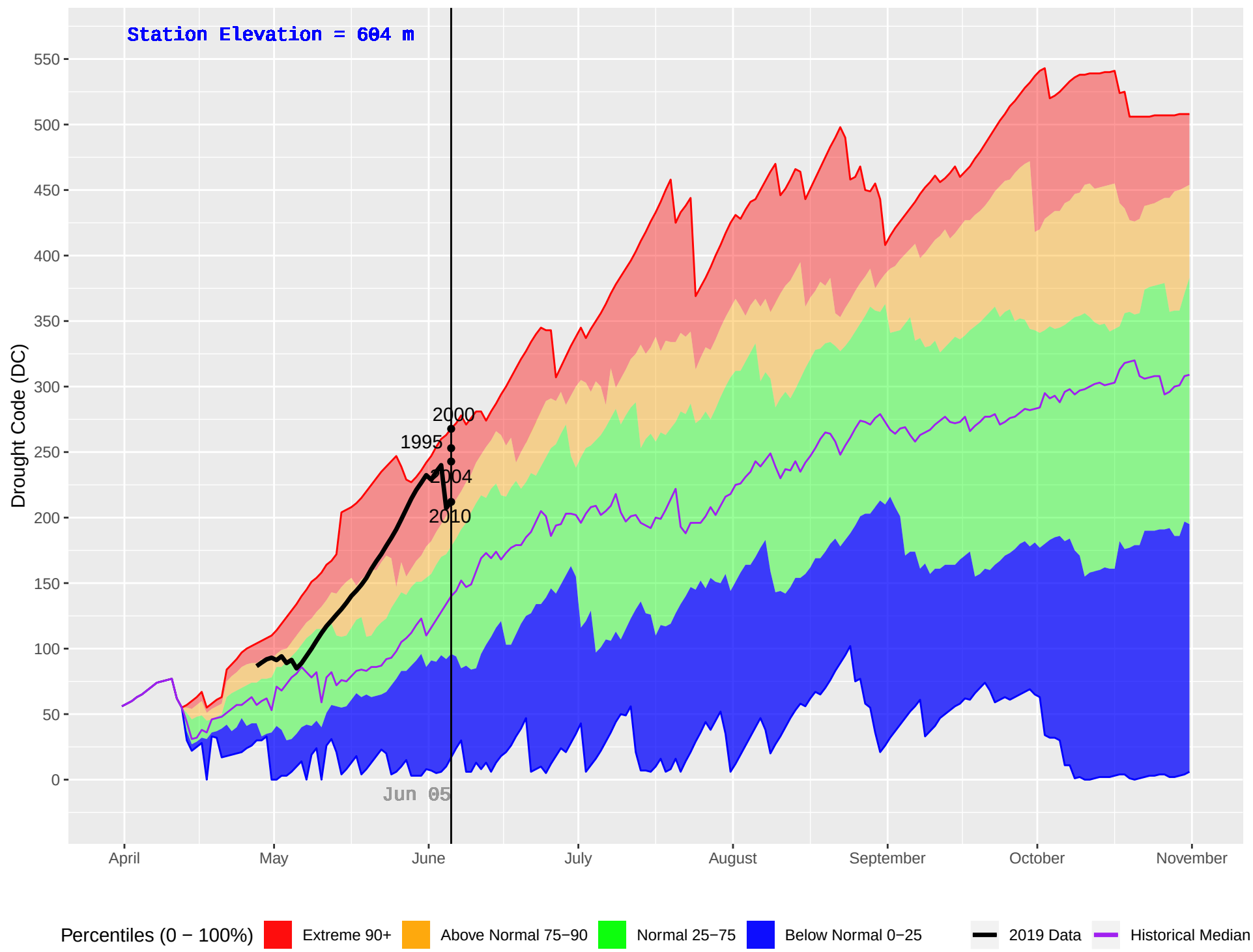
NELSON FORKS (119) : Historical (1986–2018) and Current (2019) Daily Drought Code (DC)
