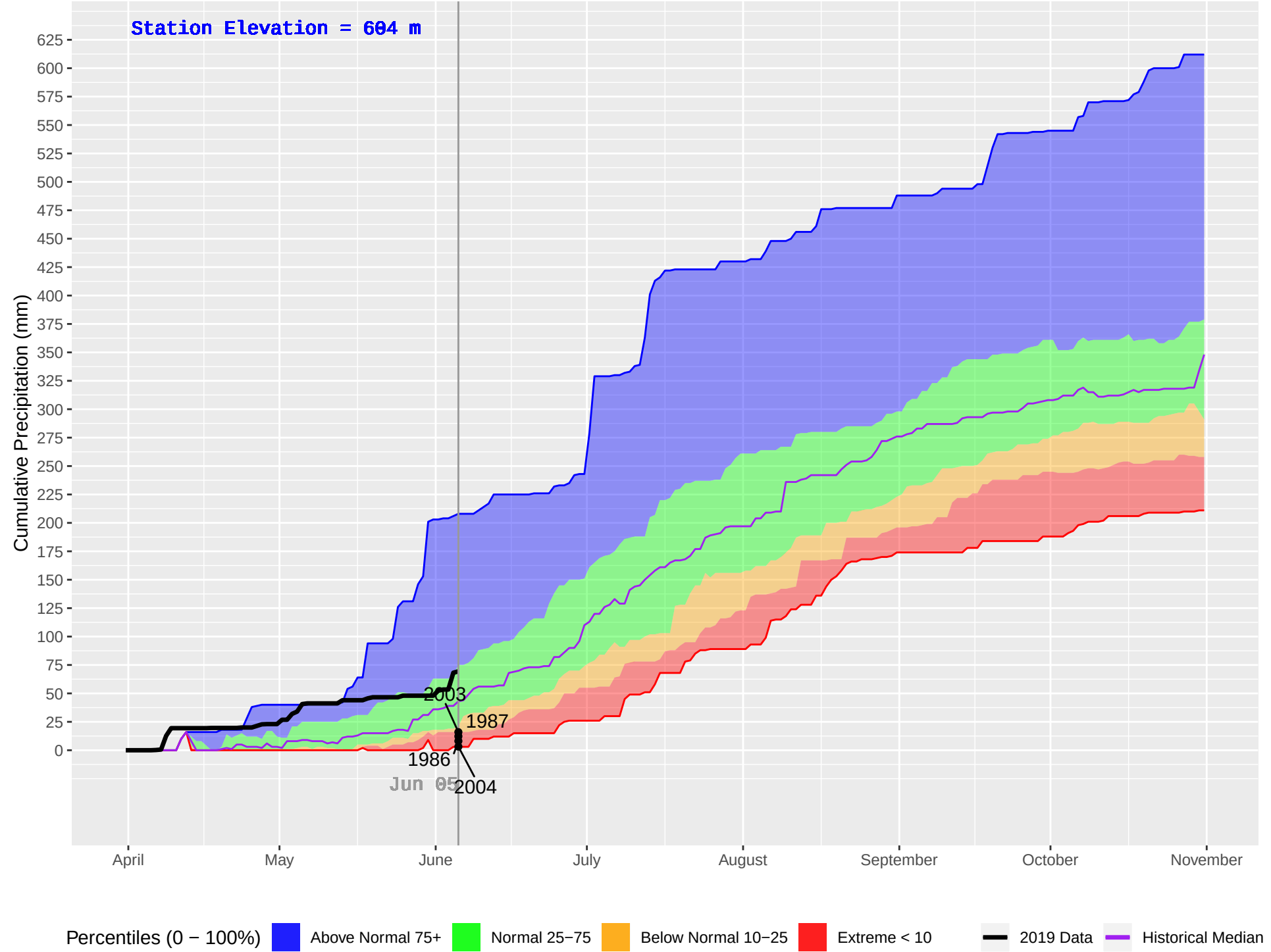
NELSON FORKS (119) : Historical (1986–2018), Current (2019) Daily Cumulative Precipitation
