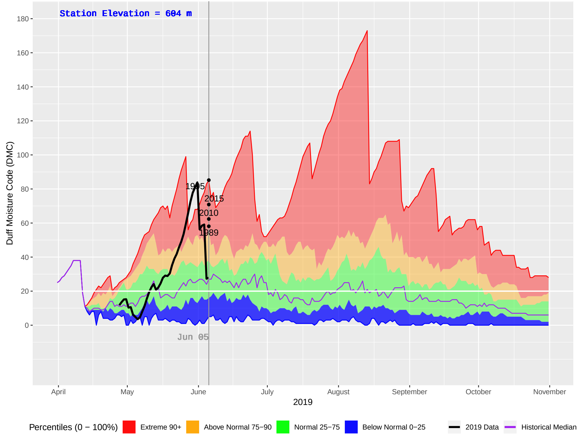
NELSON FORKS (119) : Historical (1986–2018), Current (2019) Daily Duff Moisture Code (DMC)
